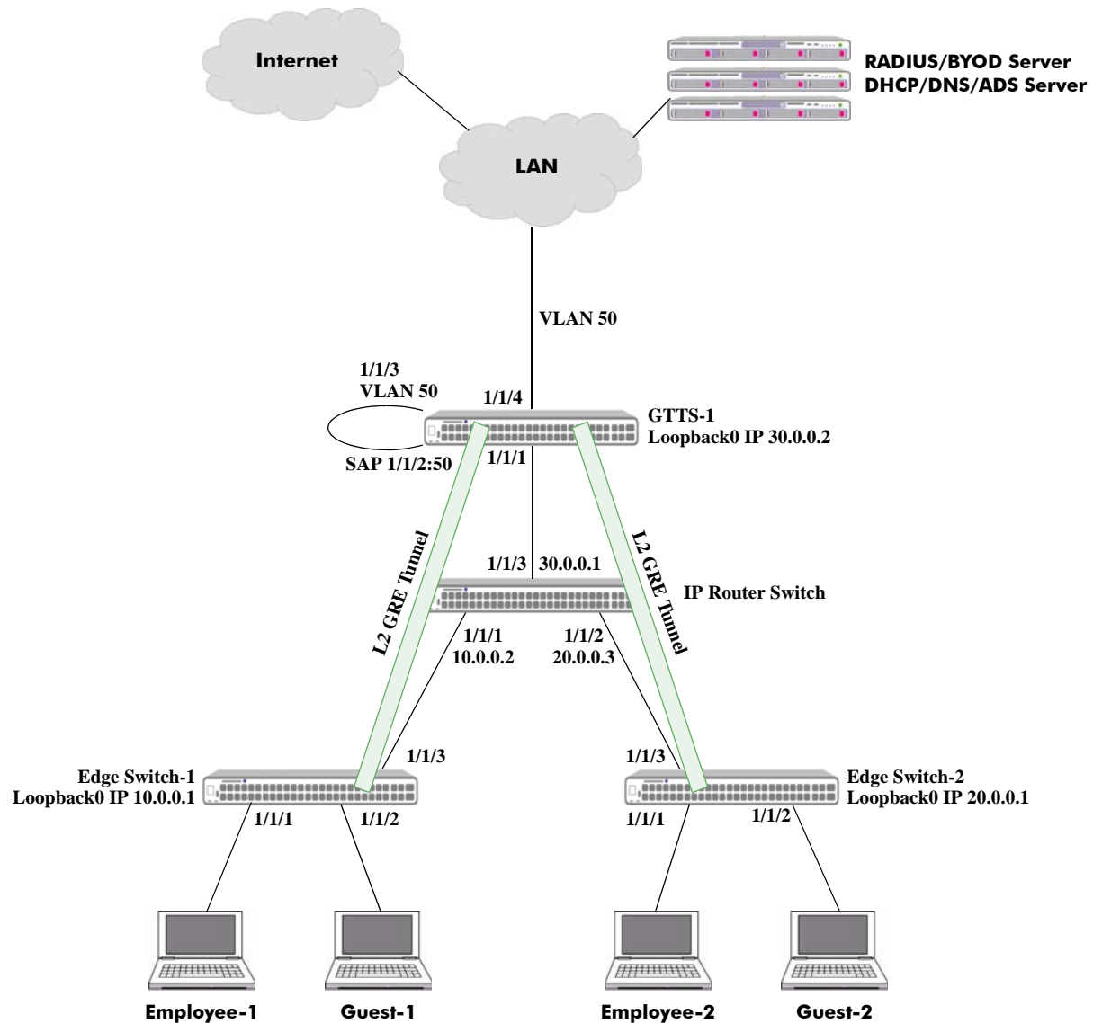
OmniSwitch Guest Tunneling Configuration Example
